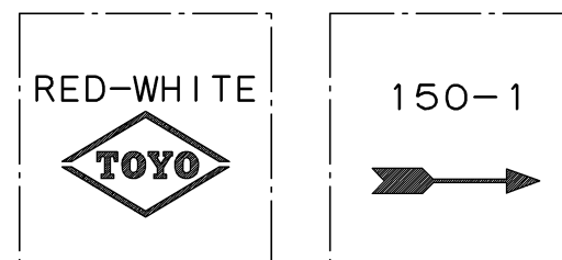
SIZES \frac{1}{2} to 3 BODY MARKING
